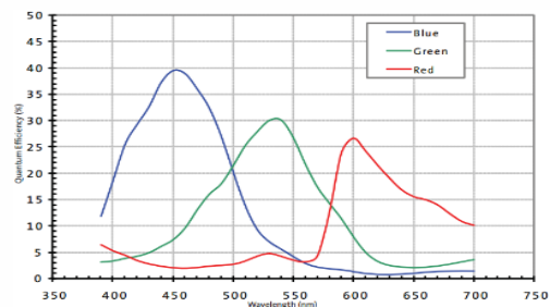
MV-CE100-30GC 量子效率
