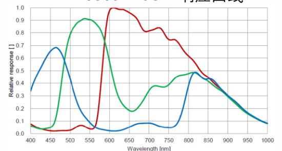
MV-CU004-10GC 响应曲线
