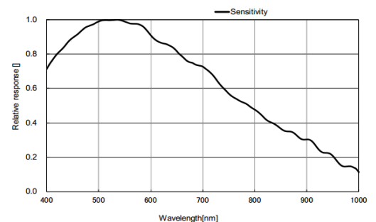
MV-CU120-10UM 量子效率
