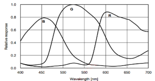
MV-CU120-10UC 量子效率
